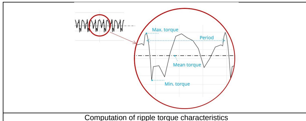
Computation of ripple torque characteristics
