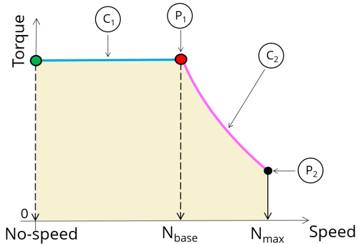
MTPA command modes – Torque-speed curve computation process
